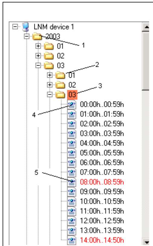
Figure 1: Data tree
