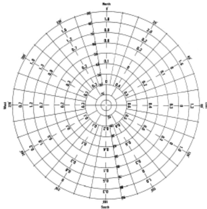
Figure 4 Polar diagram of directional response of pyranometer CM 11 810234 expressed as the percentage deviation of the ideal proportionally to the cosine of the zenith angle. The zenith axis was perpendicular to the base of the pyranometer. Orientation: cable was pointing to North.
