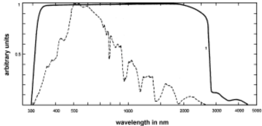
Figure 3 1. Relative spectral transmittance of two pyranometer domes. (Four surface reflections and index change with wavelength are taken into account). 2. Spectral distribution of solar radiation at sea level. Sun at zenith (Airmass 1).
