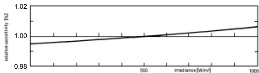
Figure 7 Non-linearity (sensitivity variation with irradiance) of Kipp & Zonen pyranometer CM 11.
