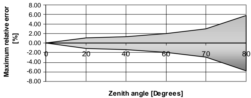
Figure 9 Relative directional error
