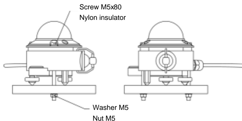
Figure 10 Mounting the pyranometer.
