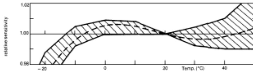
Figure 8 The curve of relative sensitivity variation with instrument temperature of a pyranometer CM 11 is in the shaded region. A typical curve is drawn.
