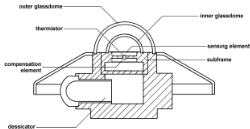
Figure 1 Approximate construction of Kipp & Zonen pyranometer CM 11.
