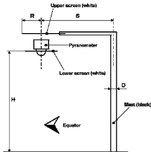
Figure 11 Arrangement to measure reflected global radiation
