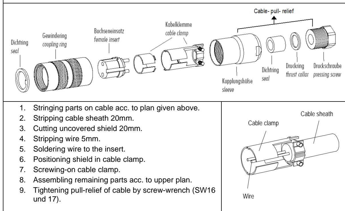
Figure 1: Plug Mounting
