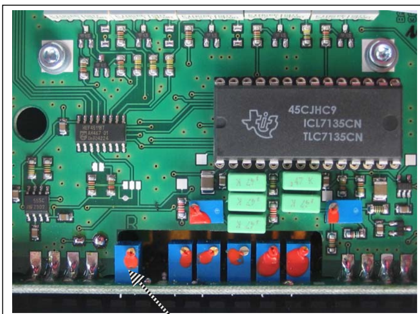
Reducing potentiometer
